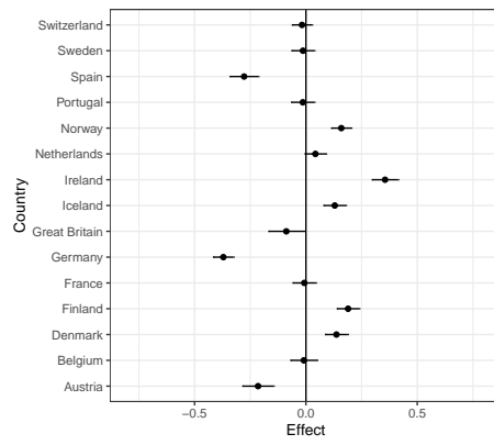
Figure 10: Constrained Country Raw Random Effects
