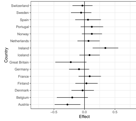
Figure 11: Nested Country Scaled Random Effects
