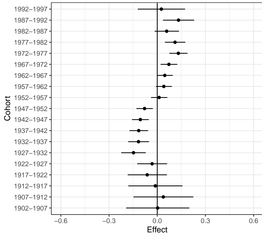
Figure 8: Nested Cohort Gender Raw Random Slopes
