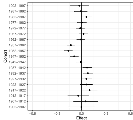
Figure 1: Predicted Constrained Raw Cohort Effects
