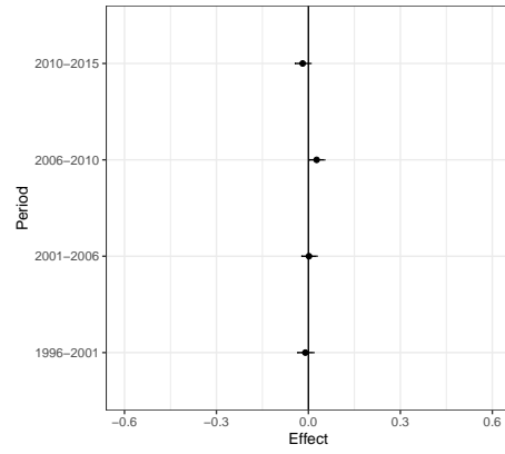
Figure 3: Predicted Constrained Raw Period Effects
